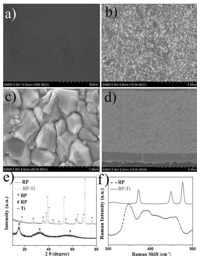
Figure 1. a) SEM image of Ti foil; b, c) SEM images of BP-Ti; d) cross-section of BP-Ti; e) XRD patterns and f) Raman spectra of BP-Ti and RP.
