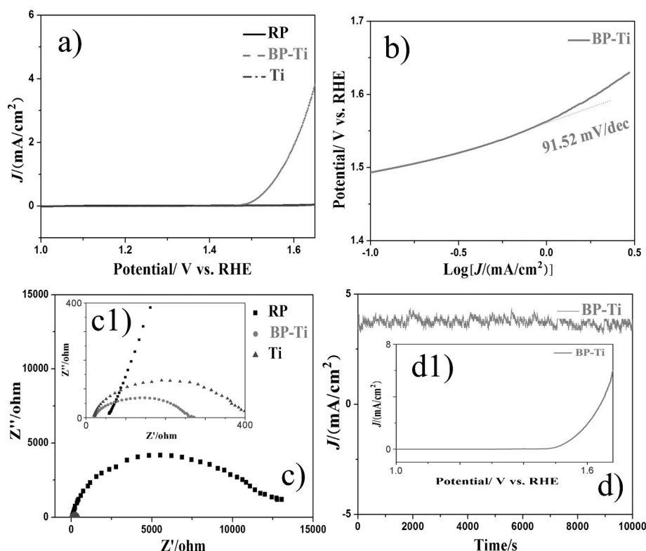
Figure 2. a) Polarization curves of RP, Ti, and BP-Ti in an O_2 -saturated KOH solution; b) Tafel plots of BP-Ti; c) electrochemical impedance spectroscopy (EIS) of RP, BP-Ti, and Ti; c1) the magnified EIS; d) chronoamperometric response at 1.65 V; d1) polarization curves of BP-Ti before chronoamperometric response.
